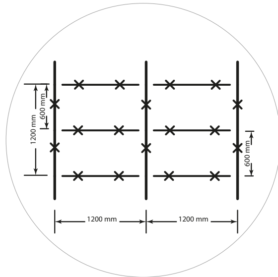
DRAWING 6
